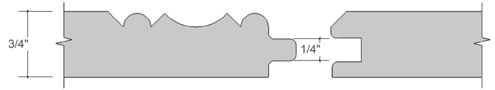
Tongue & Groove Detail
