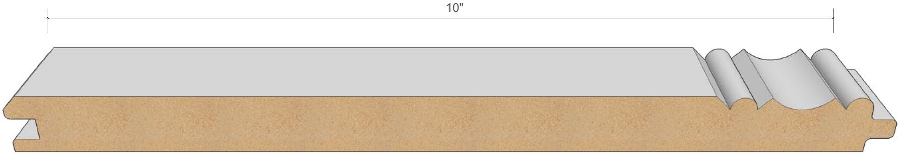
10" Finish face
