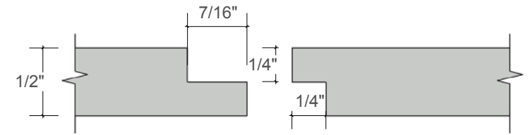
Shiplap Detail
