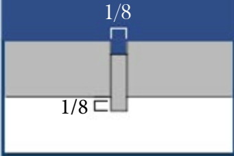
3/16" x 1/8" Channel
