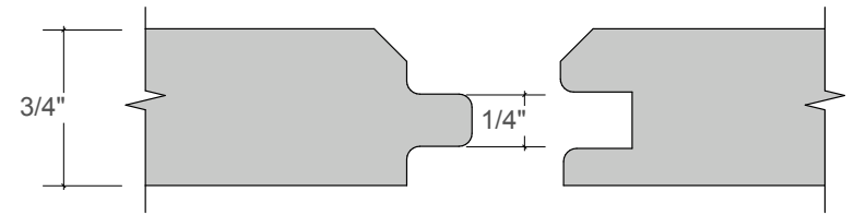
Tongue & Groove Detail
