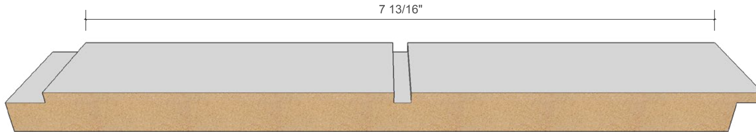
4" On-Center (8" Finish face)
