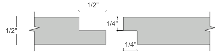
Shiplap Detail
