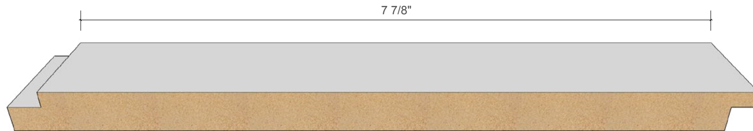
8" On-Center (8" Finish face)
