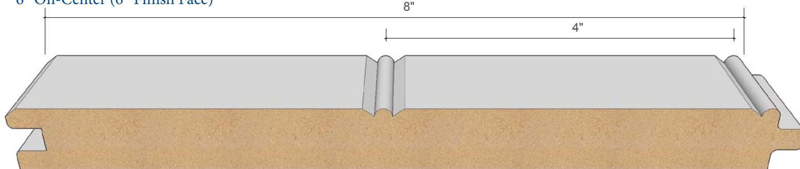
4" On-Center (8" Finish Face)
