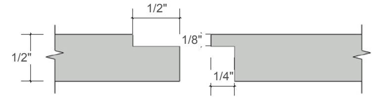
Shiplap Detail
