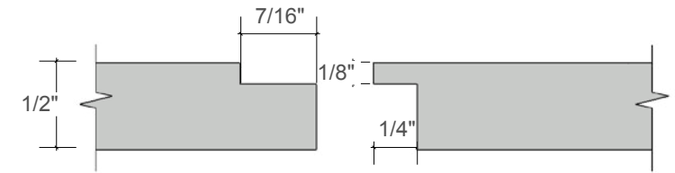
Shiplap Detail
