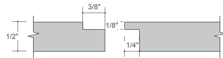
Shiplap Detail
