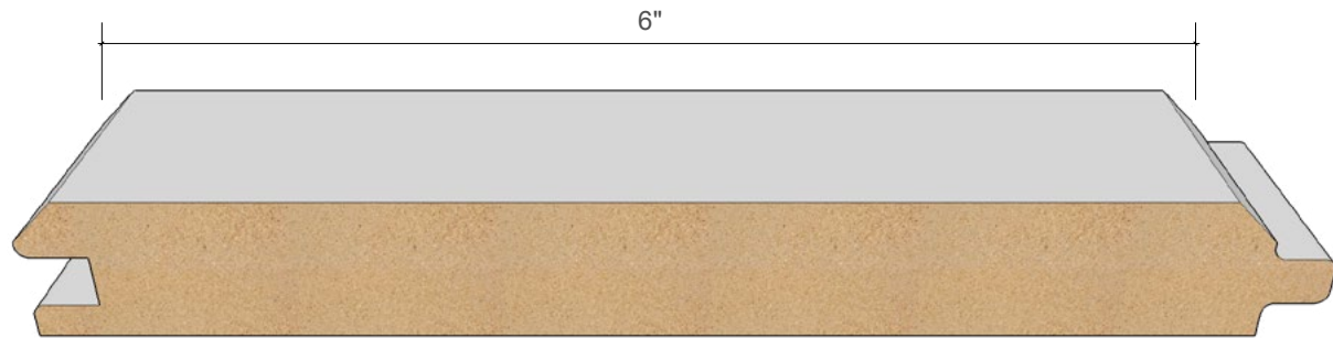
6" On-Center (6" Finish Face)
