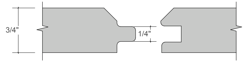
Tongue & Groove Detail
