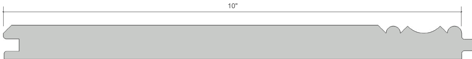
10" finish face
