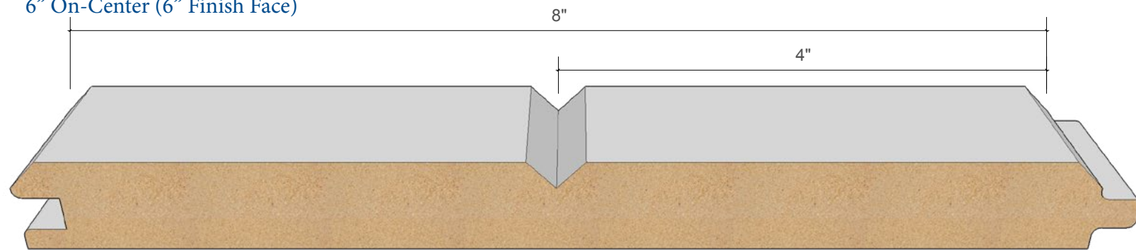
4" On-Center (8" Finish Face)
